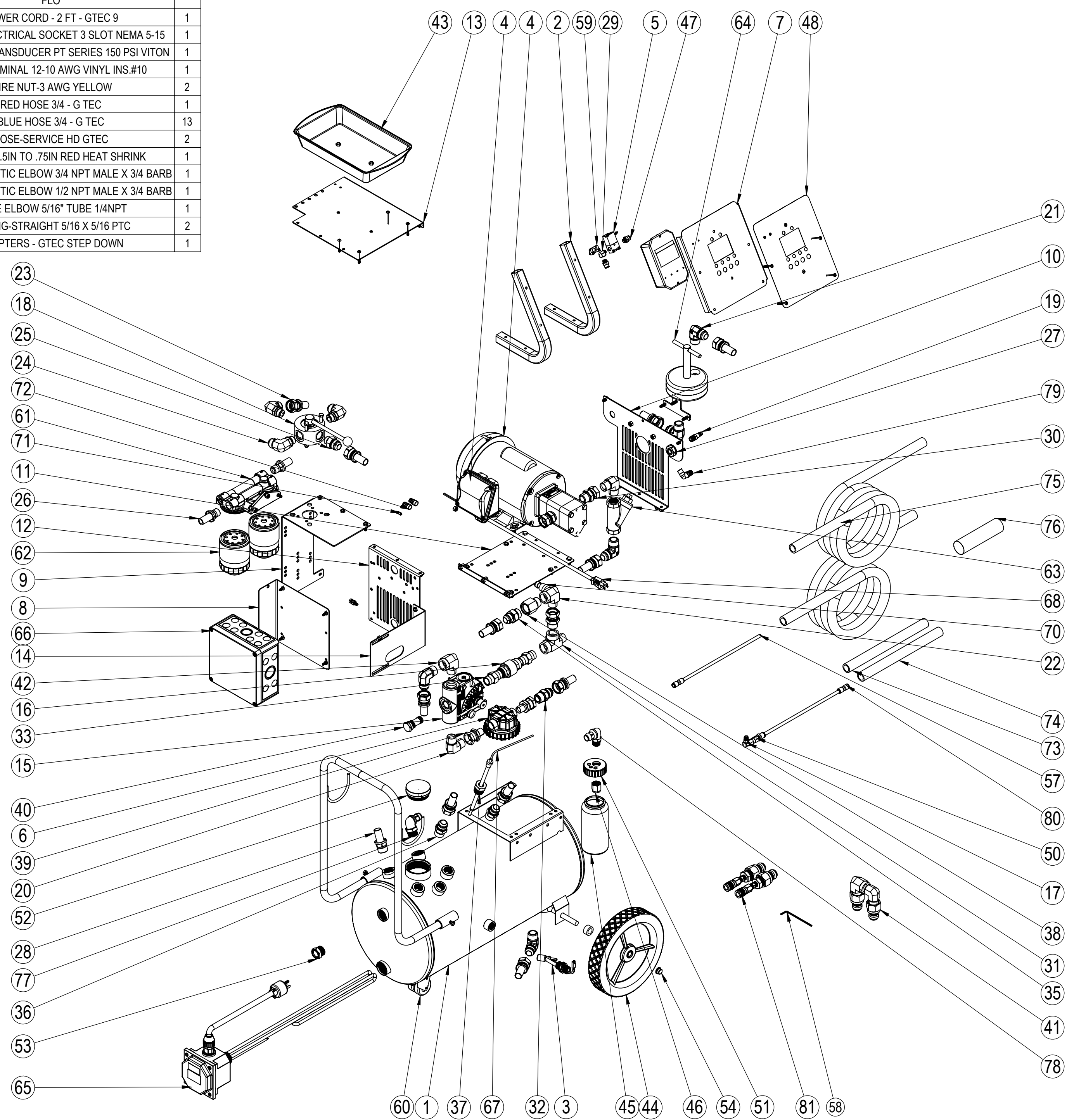
TTCF-9A PARTS BREAKDOWN
