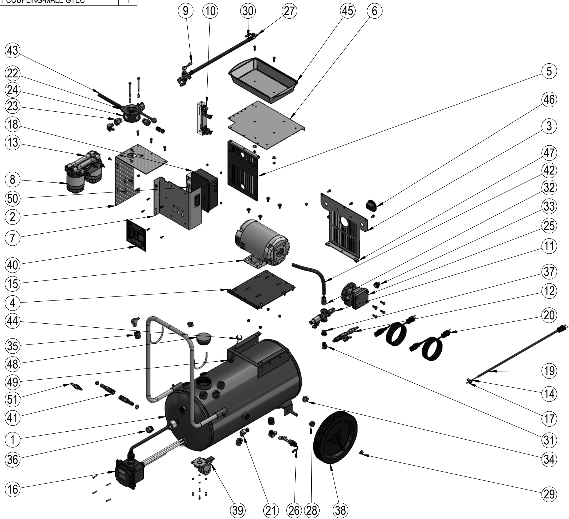
TTCF-7AR PARTS BREAKDOWN
