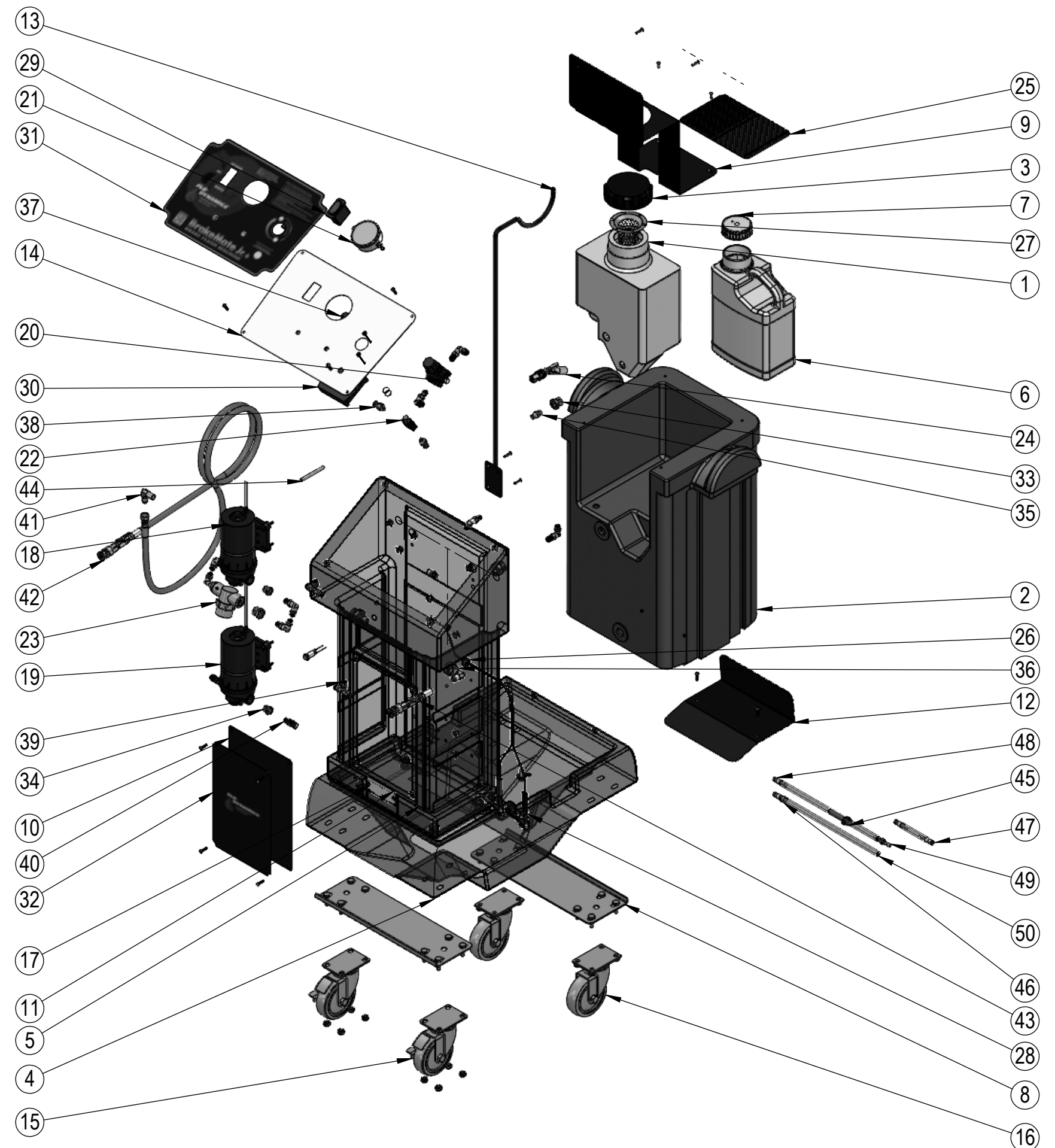
BRAKEMATE JR PLUS PARTS BREAKDOWN
